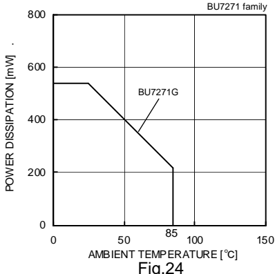
Derating curve
