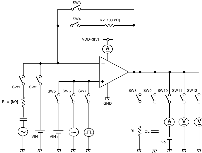
Fig.164 Test circuit 2
