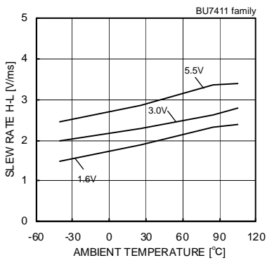
Fig.114 Slew Rate H-L – Ambient Temperature
