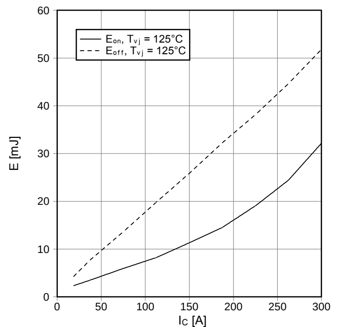
Schaltverluste IGBT-Wechselr. (typisch) switching losses IGBT-inverter (typical) E_{on} = f(I_C) , E_{off} = f(I_C) V_{GE} = \pm 15\text{ V} , R_{Gon} = 4,8\ \Omega , R_{Goff} = 4,8\ \Omega , V_{CE} = 600\text{ V}
