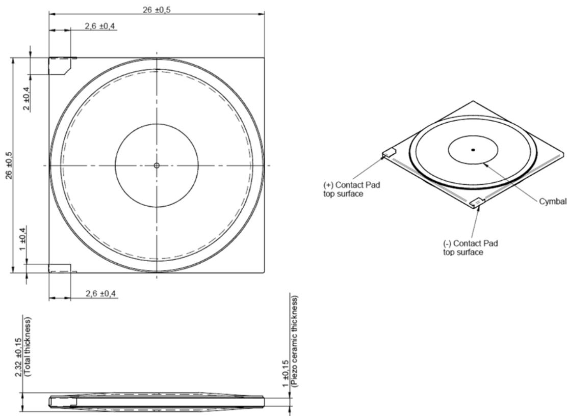
Fig. 1: Dimensional drawings
