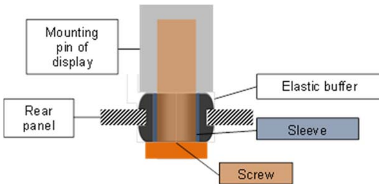
Fig. 16: Schematic drawing of a potential option for a buffer that is able to ensure movement x,y- and z-direction depending on the material and the dimension of the elastic buffer used.
