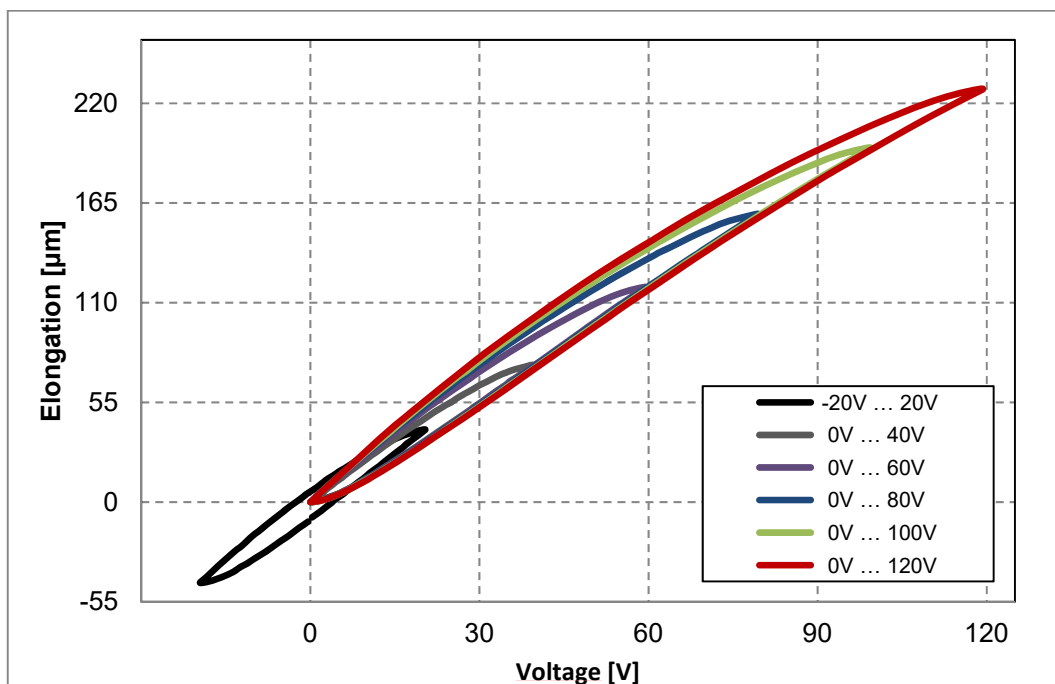
Fig. 2: Elongation as a function of voltage measured between cymbal end-caps.
