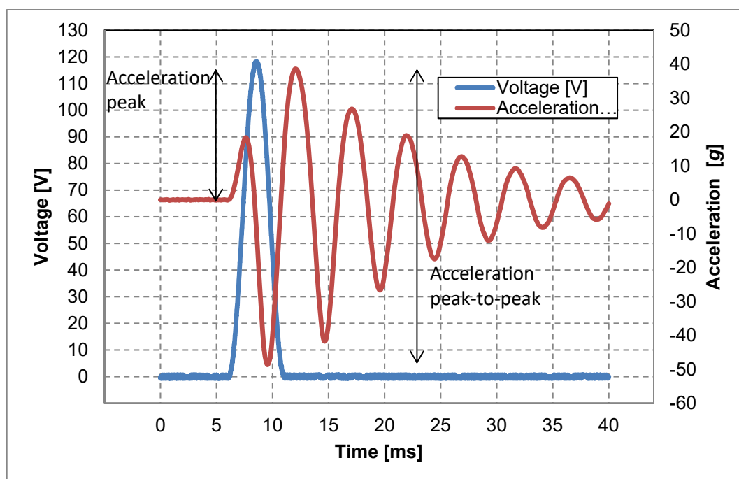
Fig. 5: Typical acceleration g as a function of input voltage with 100 g load. Input voltage with a half wave sinus signal form of amplitude 0 ... 120 V and pulse length 5 ms which is equivalent to 200 Hz.
