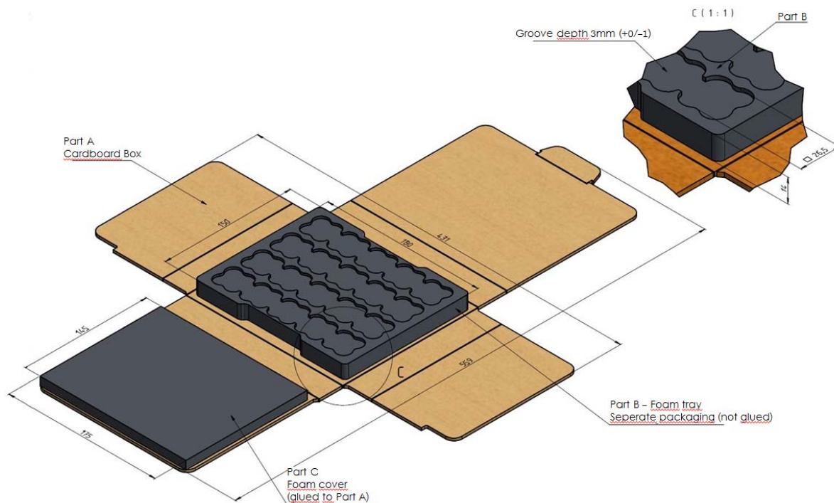
Fig. 18: Drawing of the packaging unit.
