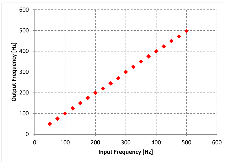
Fig. 8: Output frequency of acceleration vs. input voltage signal frequency for 10 pulses. Input voltage has a single pulse half wave sinus signal form of amplitude 0 ... 120 V and varying frequency from 50 ... 500 Hz. The frequency of output acceleration is calculated.
