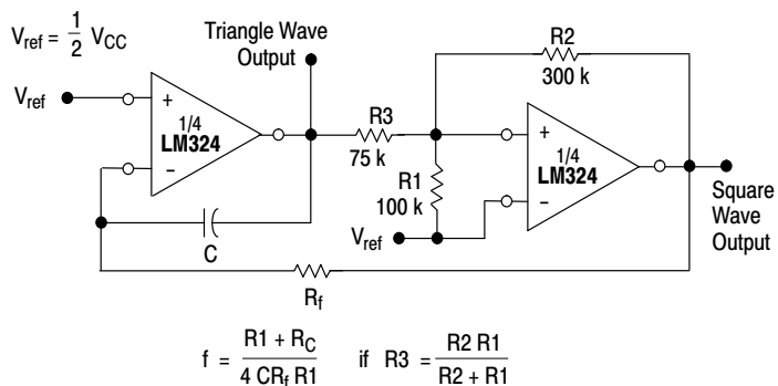
Figure 16. Function Generator
