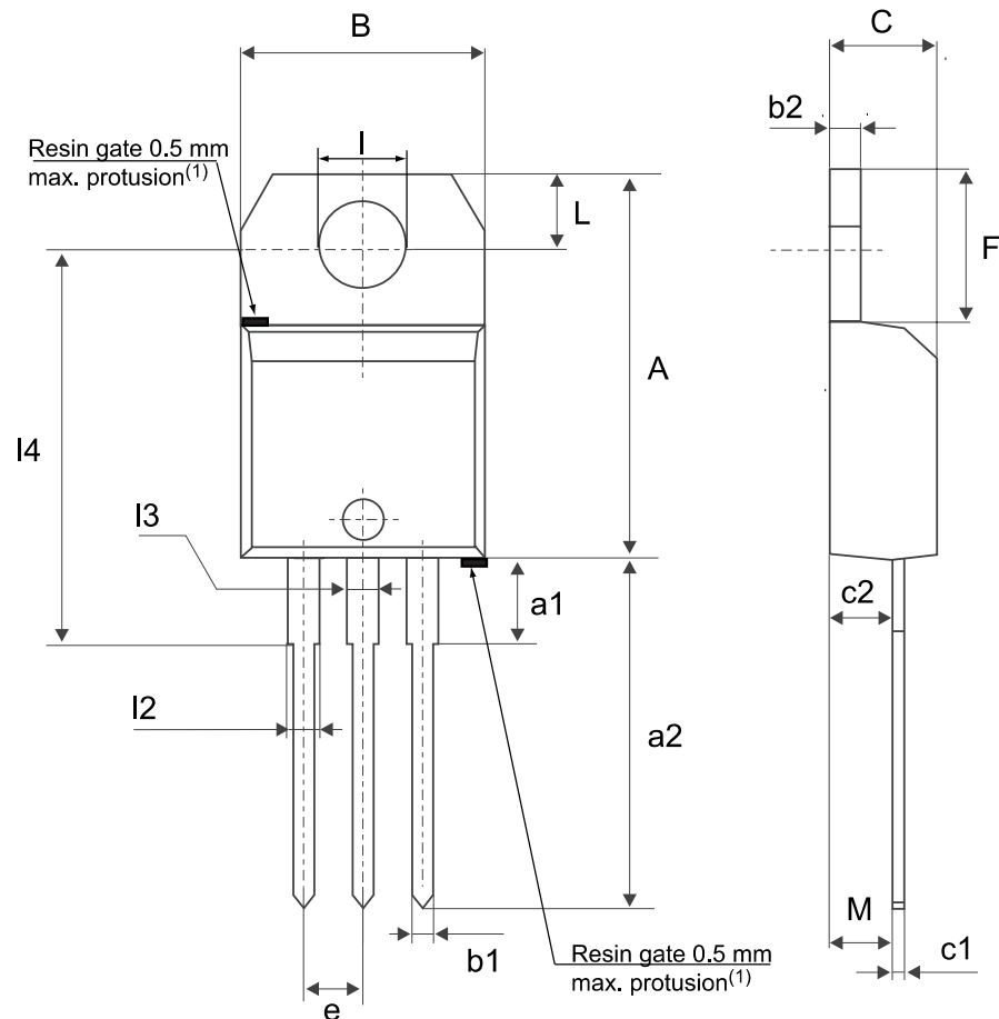
Figure 13. TO-220AB package outline
