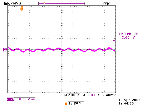
Figure 10: Output ripple & noise at 12Vin, 2.5V/40A out (10mv/div, 2µS/div)
