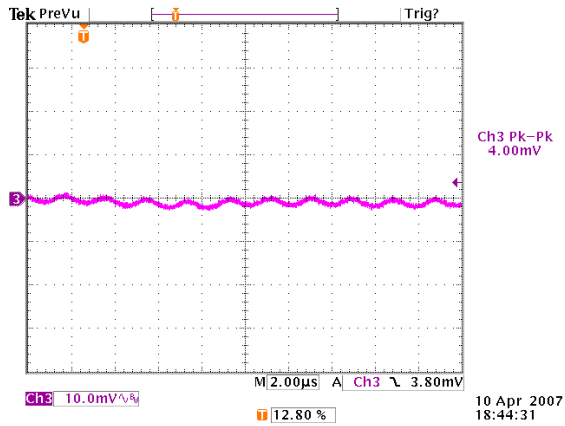
Figure 9: Output ripple & noise at 12Vin, 1.8V/40A out (10mv/div, 2µS/div)
