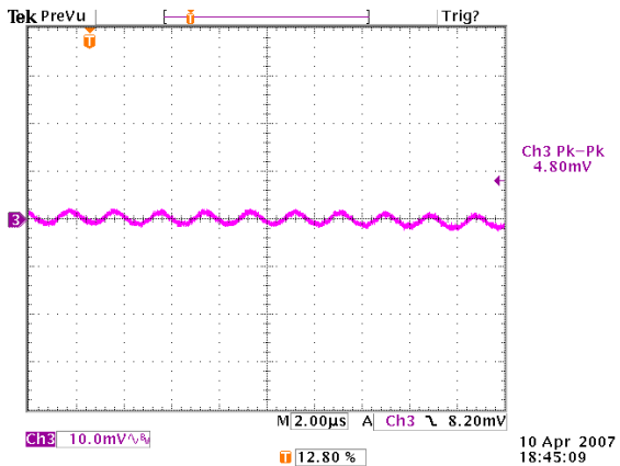
Figure 11: Output ripple & noise at 12Vin, 3.3V/40A out (10mv/div, 2µS/div)
