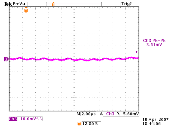
Figure 8: Output ripple & noise at 12Vin, 1.2V/40A out (10mv/div, 2µS/div)
