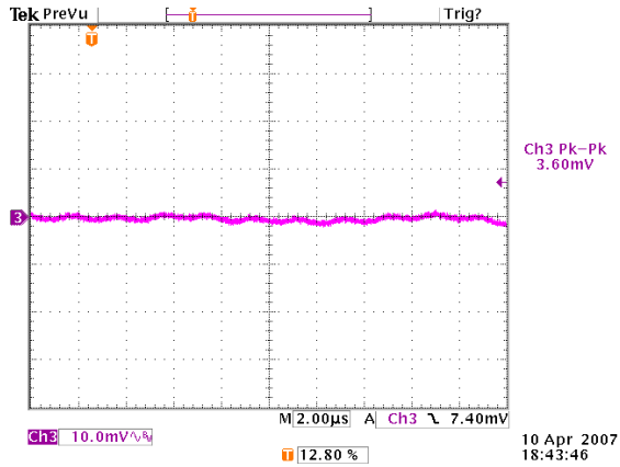
Figure 7: Output ripple & noise at 12Vin, 0.9V/40A out (10mv/div, 2µS/div)
