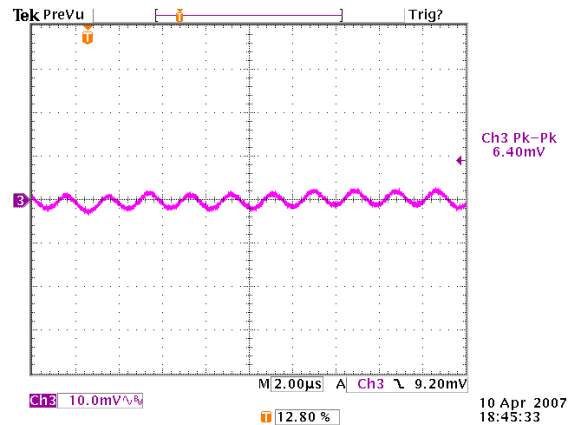
Figure 12: Output ripple & noise at 12Vin, 5.0V/40A out (10mv/div, 2µS/div)
