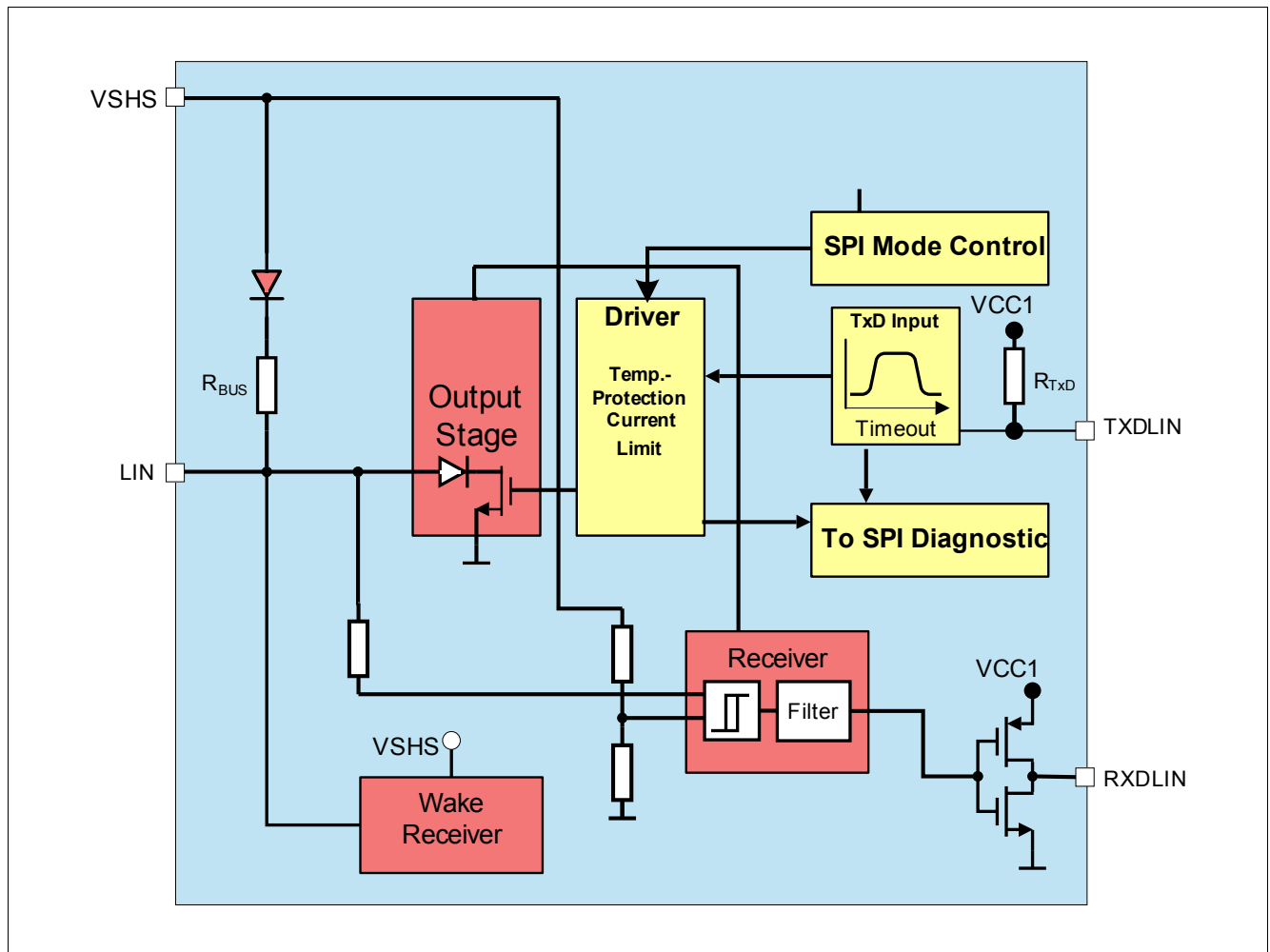
Figure 32 Block Diagram
