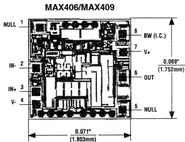
TRANSISTOR COUNT: 148; SUBSTRATE CONNECTED TO V+.
