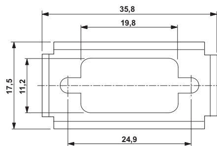
D-SUB panel mounting frame
