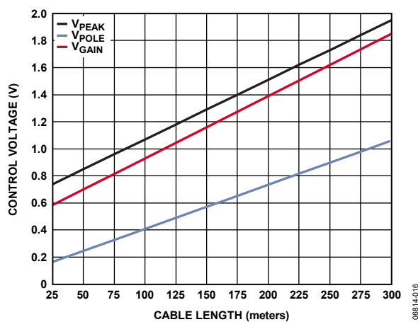
Figure 18. Recommended Settings for Coaxial Cable
