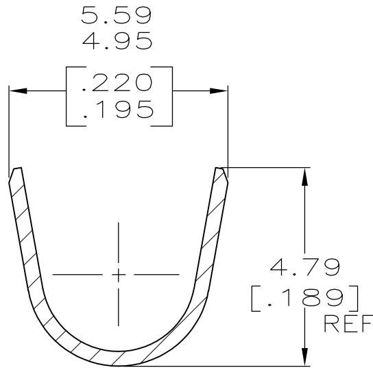
SECTION C-C SCALE 8:1
