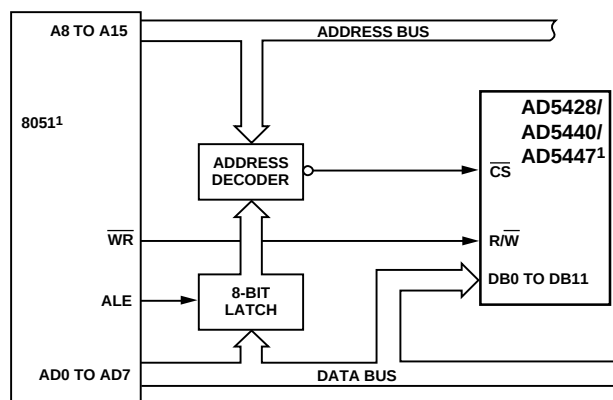
Figure 45. 8xC51-to-AD5428/AD5440/AD5447 Interface
