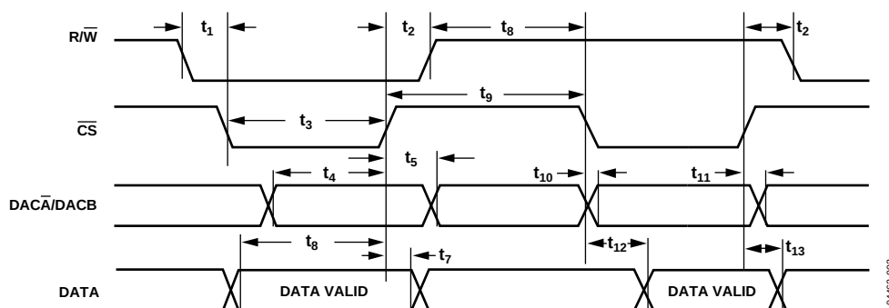
Figure 2. Timing Diagram
