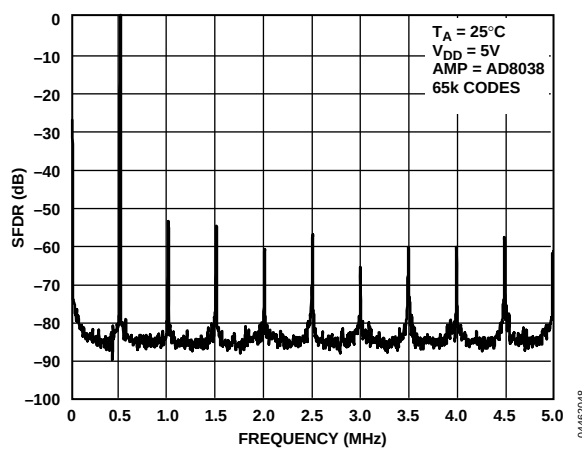
Figure 30. Wideband SFDR, f_{OUT} = 500 kHz, Clock = 10 MHz
