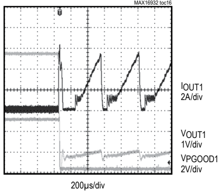
SHORT CIRCUIT RESPONSE
