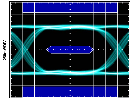
0.125UI/DIV AT 2.25Gbps Figure 7. Rx Eye Diagram at TP3, EQ = 12 dB (Cable = 2 Meters, 24 AWG, Data Rate = 2.25 Gbps)
