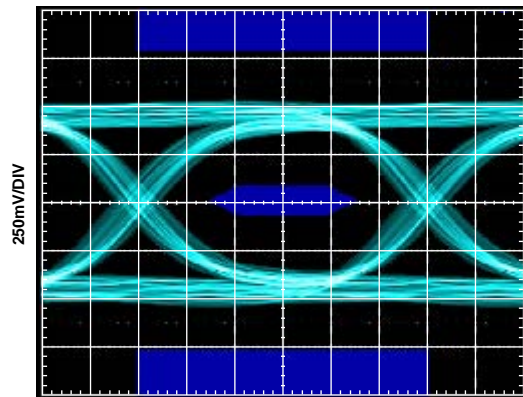
0.167UI/DIV AT 3.0Gbps Figure 8. Rx Eye Diagram at TP3, EQ = 12 dB (Cable = 2 Meters, 24 AWG, Data Rate = 3 Gbps)
