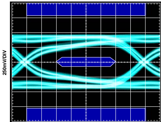
0.125UI/DIV AT 2.25Gbps Figure 5. Rx Eye Diagram at TP2 (Cable = 2 Meters, 24 AWG, Data Rate = 2.25 Gbps)
