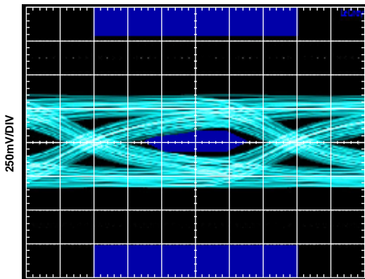
0.167UI/DIV AT 3.0Gbps Figure 6. Rx Eye Diagram at TP2 (Cable = 2 Meters, 24 AWG, Data Rate = 3 Gbps)
