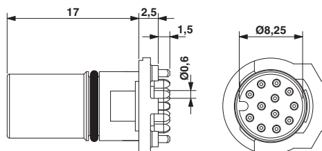
M12 flush-type connector
