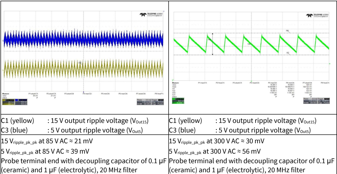
Figure 24 Output ripple voltage at ABM 0.8 W load
