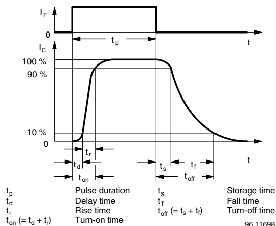
Fig. 2 - Switching Times
