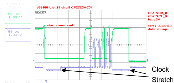
Figure 14. Example waveforms showing clock stretching.
