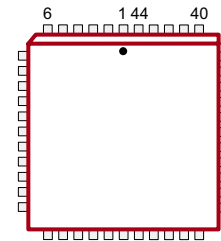
44-Lead PLCC (PJ) (top view)
