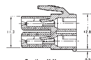
Section X-X
