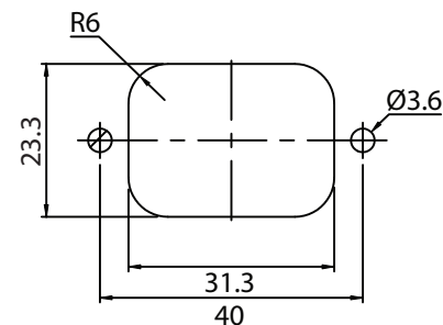
PANEL CUTOUT
