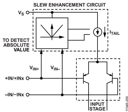
Figure 51. Slew Enhancement Circuit
