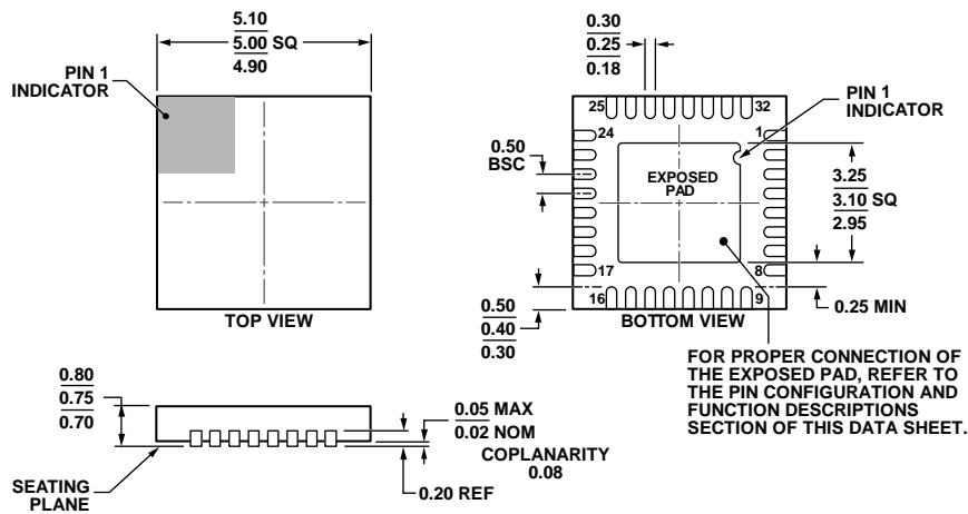
Figure 30. 32-Lead Lead Frame Chip Scale Package [LFCSP_WQ] 5 mm × 5 mm Body, Very Very Thin Quad (CP-32-7)
