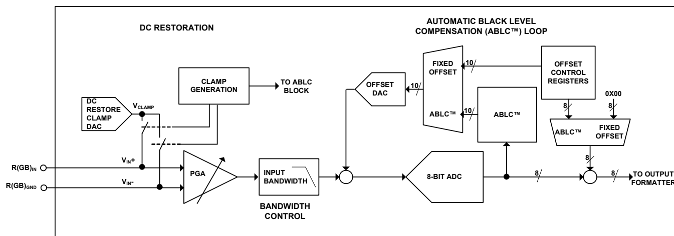
FIGURE 5. VIDEO FLOW (INCLUDING ABLC™)
