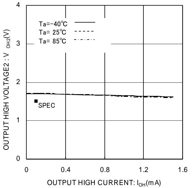
Figure 9. Output high voltage2 V_{OH2} ( V_{CC}=1.7\text{V} )
