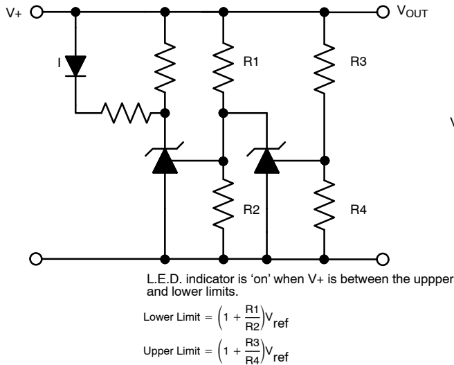
Figure 30. Voltage Monitoring
