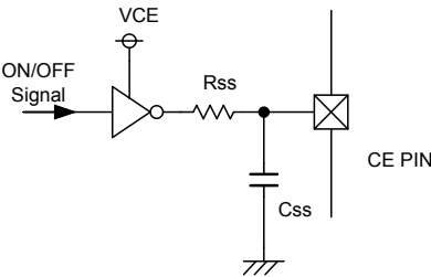
> Circuit Examl2 : CMOS logic (low current dissipation)
