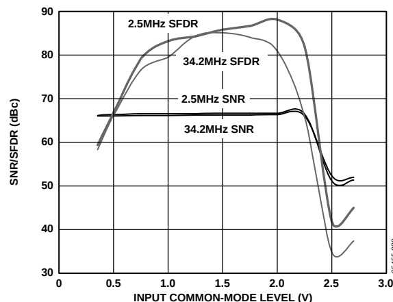
Figure 34. AD9237-65 SNR/SFDR vs. Input Common-Mode Level
