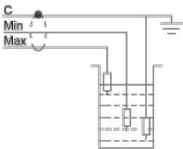
Wiring Diagram
