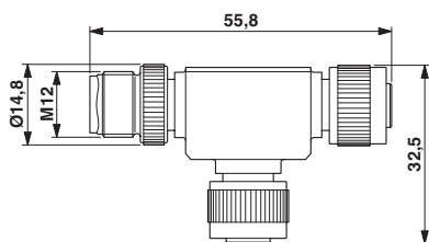
M12 T-distributor
