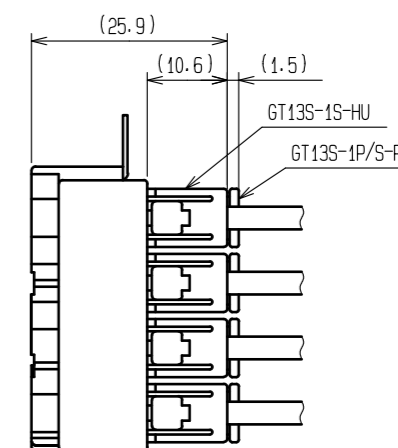
MATED CONNECTOR
