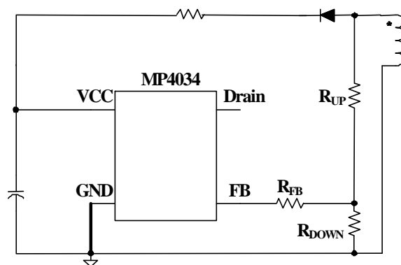
Figure 12: FB Pin in Series with ON Resistor
