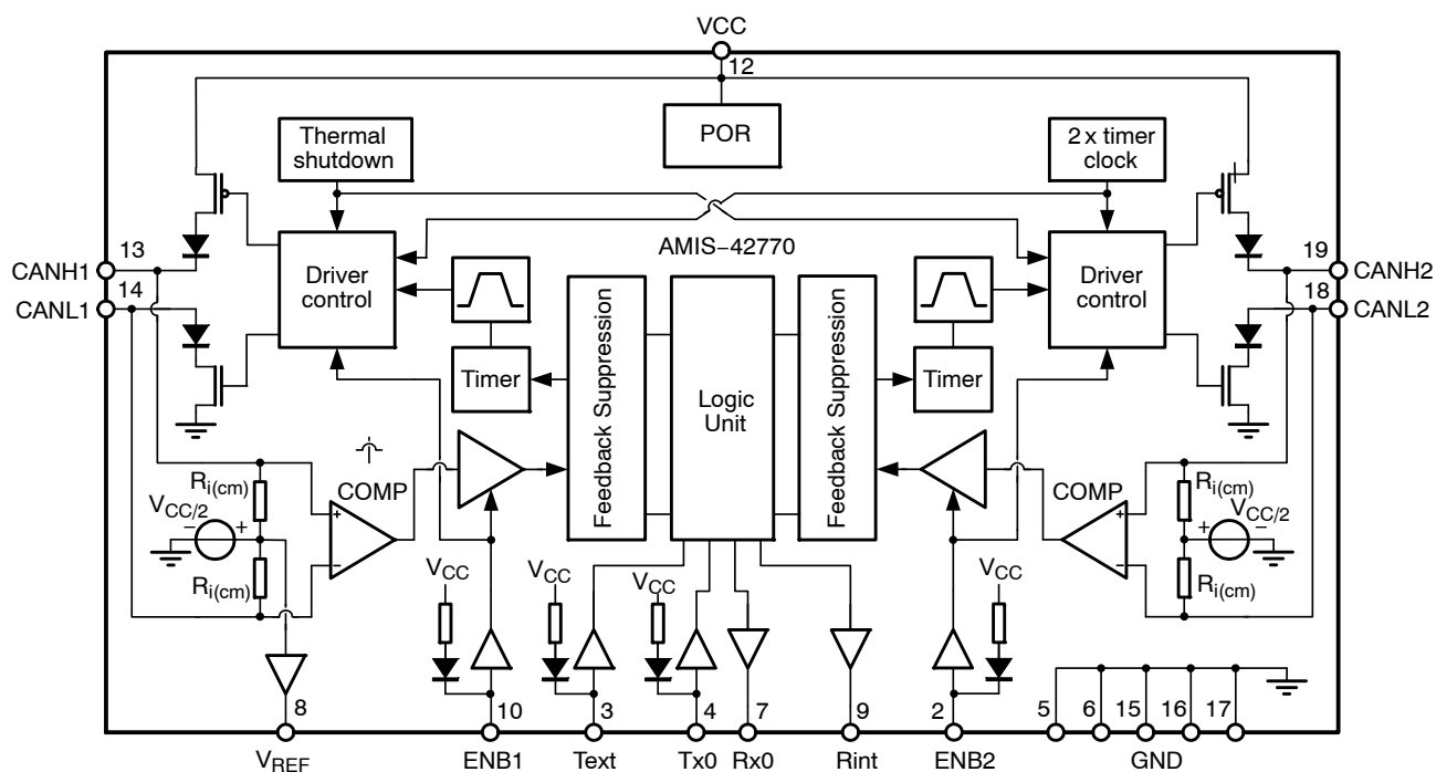
Figure 1. Block Diagram
