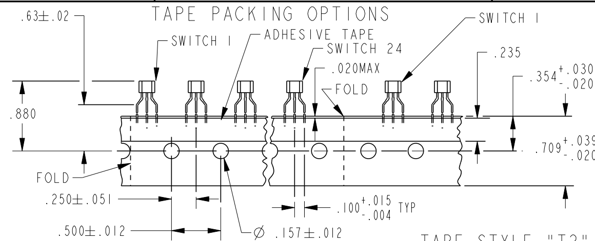
TAPE STYLE "T2"
