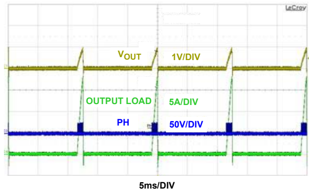
FIGURE 20. SHORT PROTECTION
