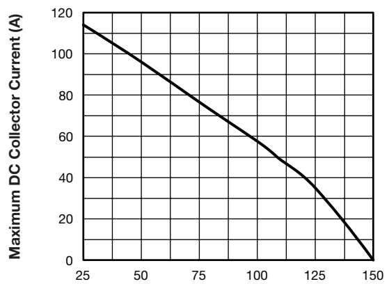
94468_02 T C - Case Temperature (°C) Fig. 2 - Maximum Collector Current vs. Case Temperature
