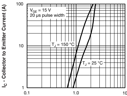
94468_01 V CE - Collector to Emitter Voltage (V) Fig. 1 - Typical Output Characteristics
