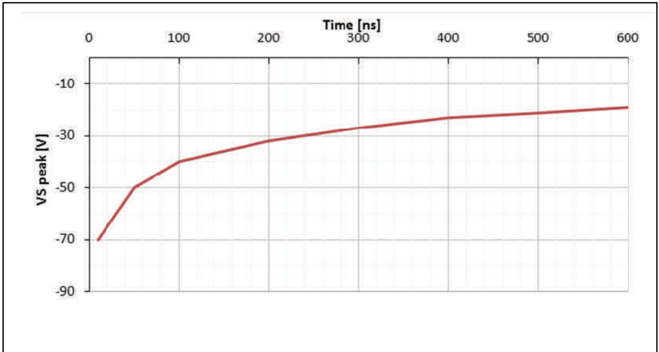
Figure 17 Negative transient Vs SOA for integrated gate driver
