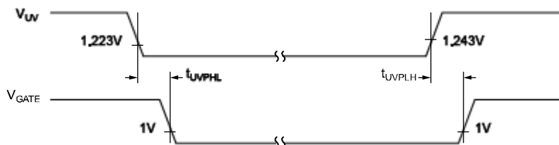
Figure 4. MIC2589/MIC2595R Undervoltage Response
