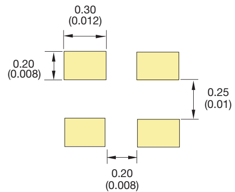
CP0302
