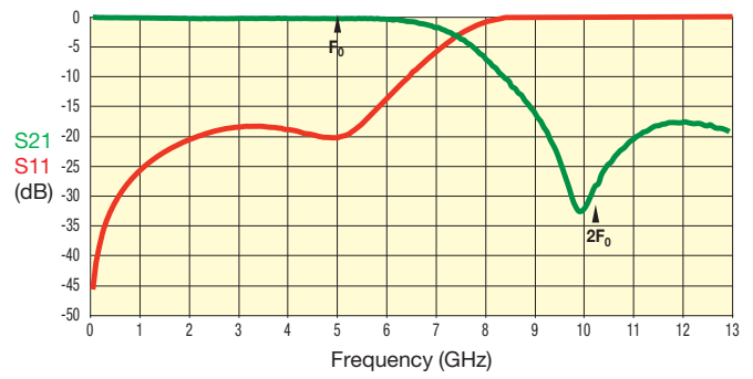
LP0603N5200ANTR
