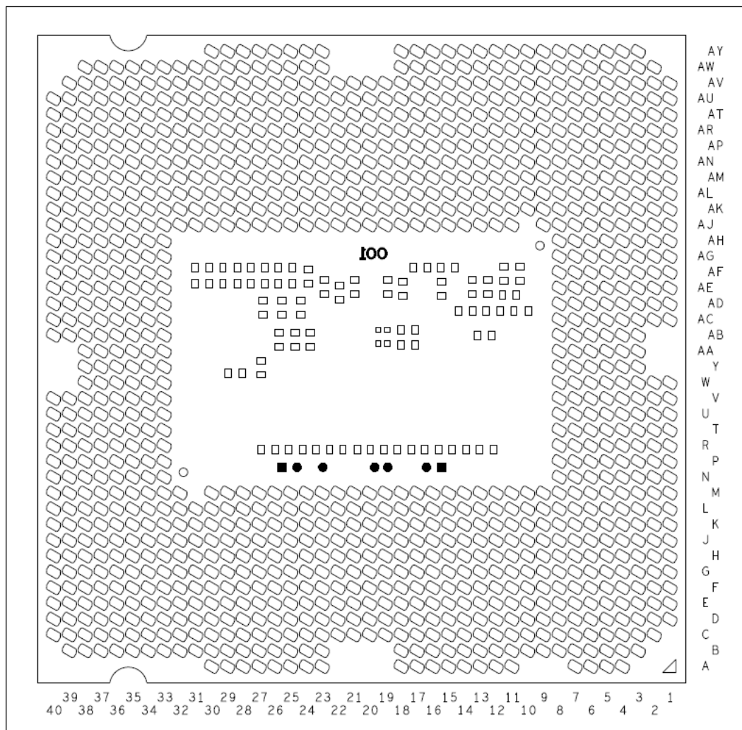
Figure 26. Processor Package Land Coordinates
