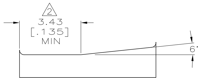
CRIMP CONFIGURATION
