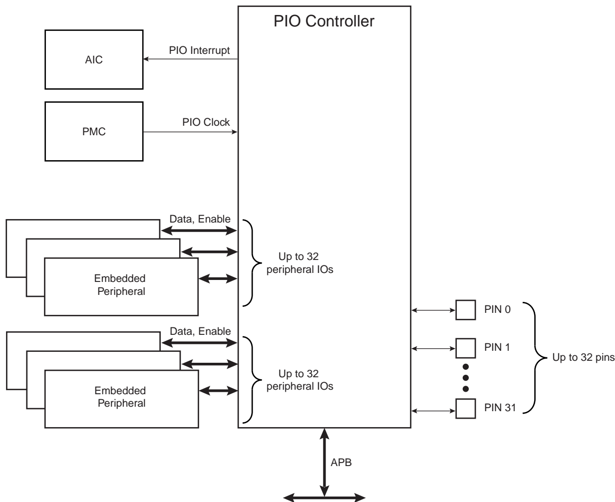
Figure 30-1. Block Diagram
