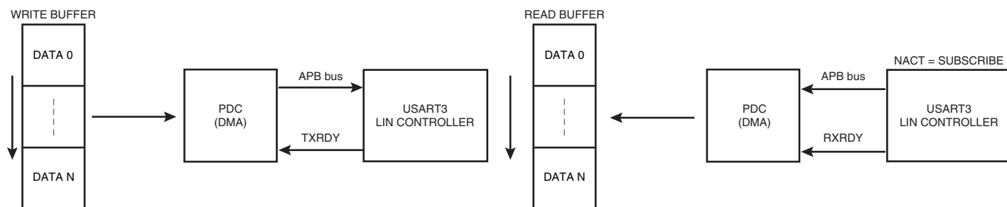
Figure 33-54. Slave Node with PDC
