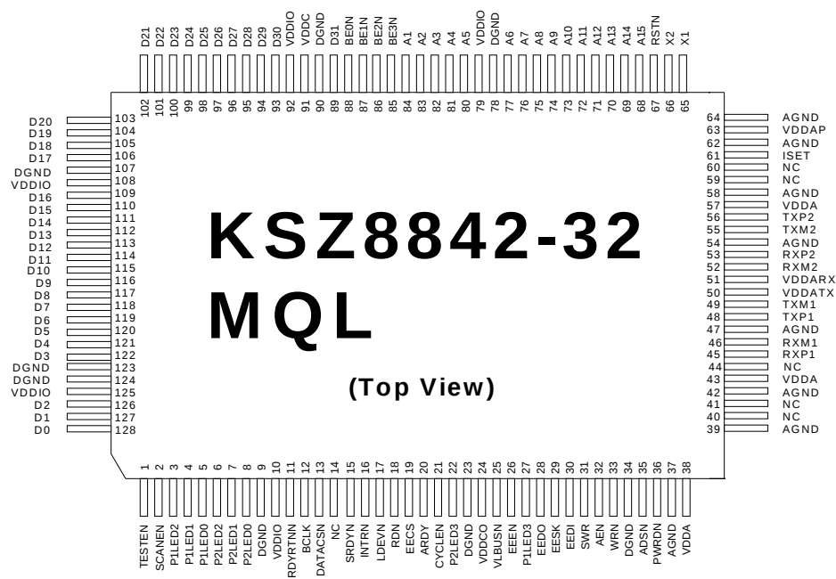
Figure 5. Standard – KSZ8842-32 MQL 128-Pin PQFP (Top View)
