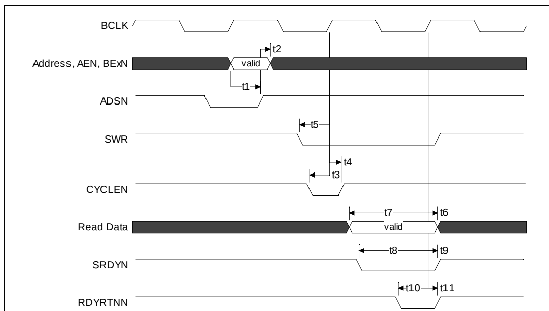
Figure 24. Synchronous Read Cycle – VLBSN = 0
