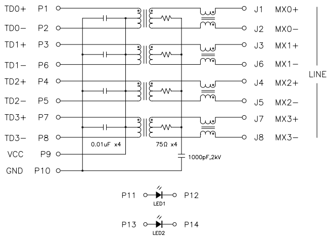
Circuit C
