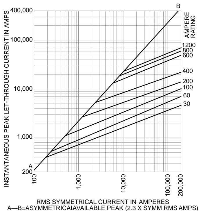
Current-Limitation Curves
