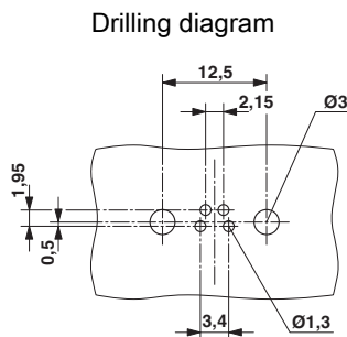
Drilling diagram
